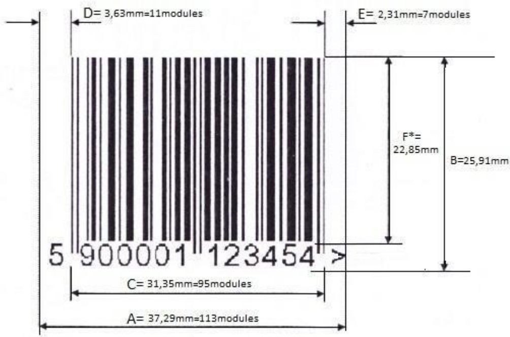
Fig 2. Nominal dimension for EAN-13 bar code (the magnification factor 1.0)
