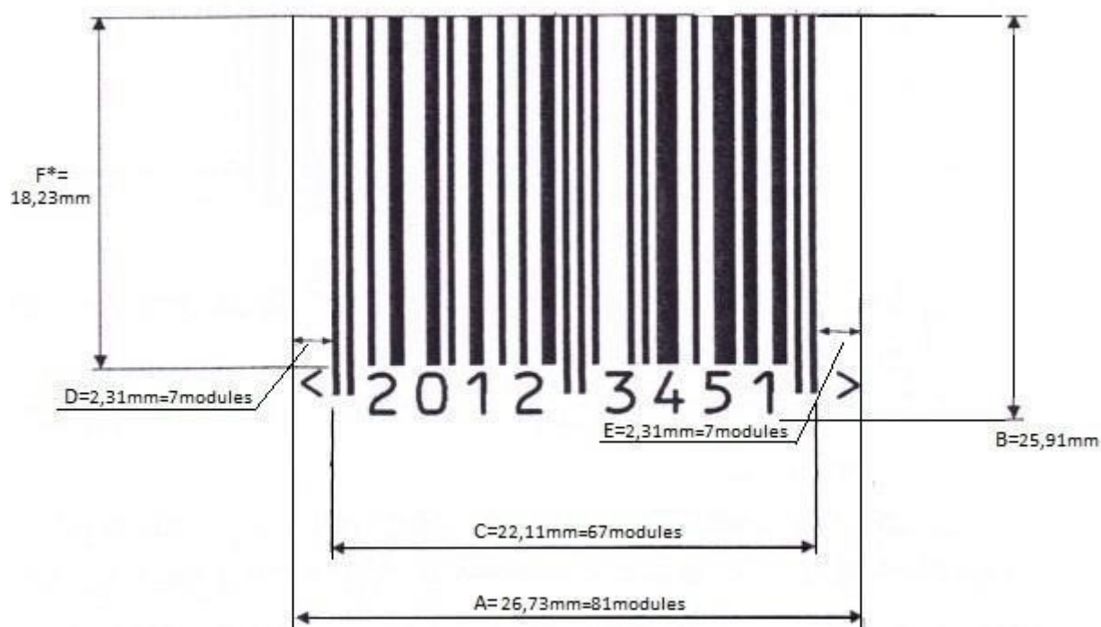
Fig 4. Nominal dimension bar code EAN-8 for the magnification factor 1.0
